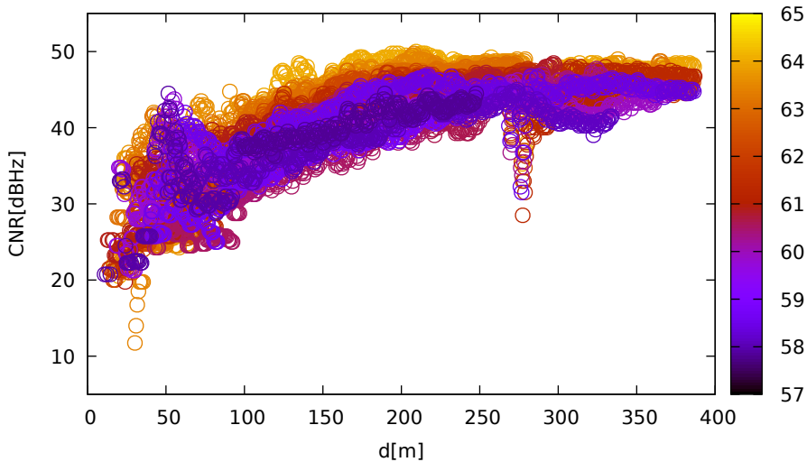
CNR vs distance (Javad for E33 at L1)
