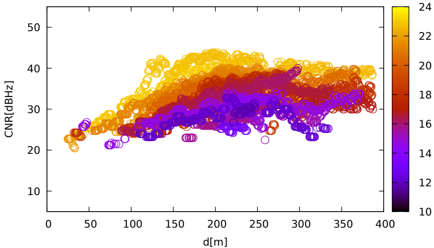
CNR vs distance (Javad for G02 at L1)
