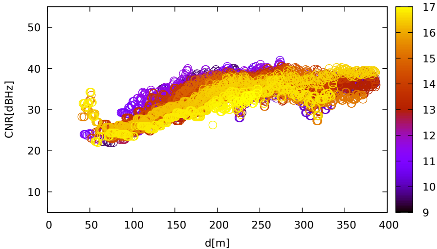
CNR vs distance (Javad for G05 at L1)
