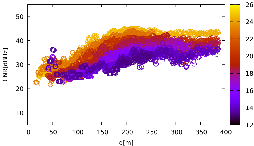
CNR vs distance (Javad for G12 at L1)
