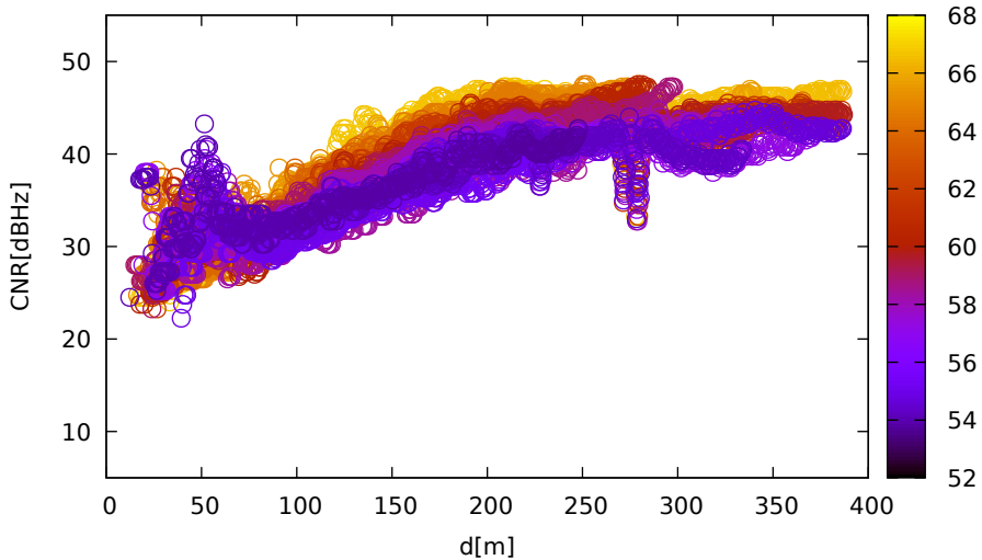
CNR vs distance (Javad for G25 at L1)
