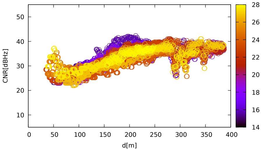
CNR vs distance (Javad for G26 at L1)
