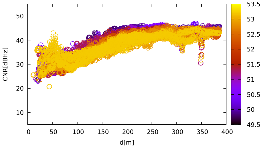
CNR vs distance (Javad for G31 at L1)
