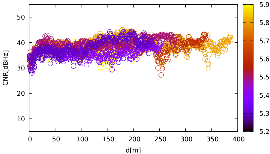
CNR vs distance (Javad for R03 at L1)
