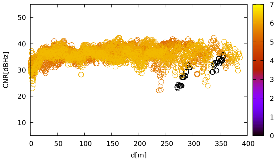
CNR vs distance (Javad for R04 at L1)
