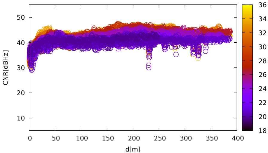
CNR vs distance (Javad for R10 at L1)
