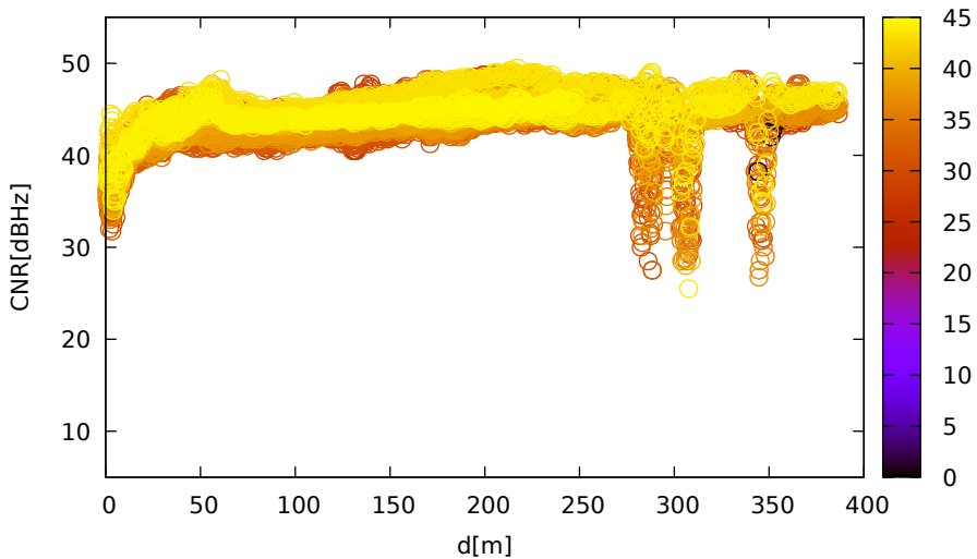
CNR vs distance (Javad for R12 at L1)
