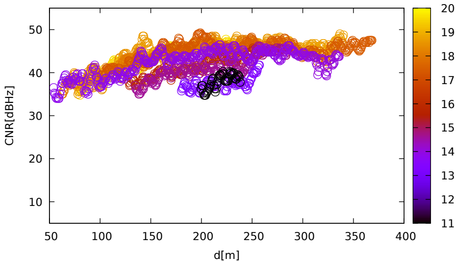
CNR vs distance (LeicaGS15 for E01 at L1)
