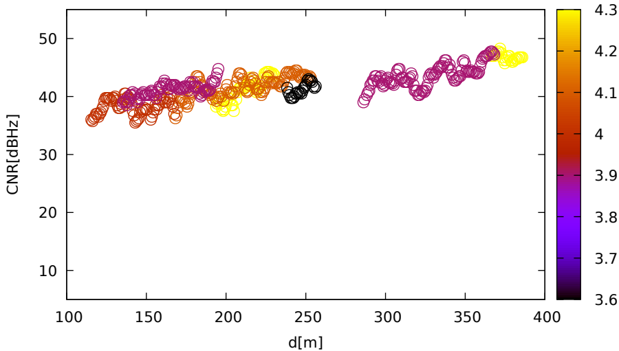
CNR vs distance (LeicaGS15 for E03 at L1)
