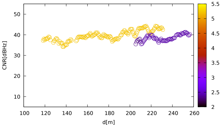
CNR vs distance (LeicaGS15 for E05 at L1)
