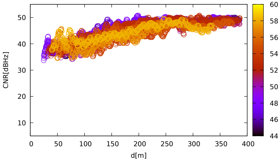
CNR vs distance (LeicaGS15 for E12 at L1)
