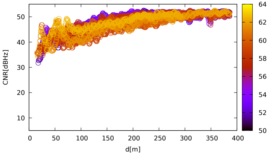
CNR vs distance (LeicaGS15 for E24 at L1)
