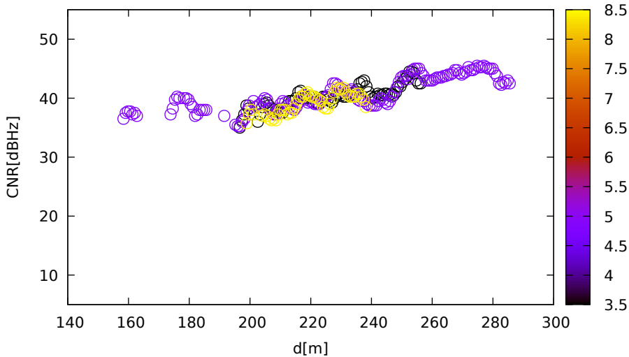
CNR vs distance (LeicaGS15 for E25 at L1)
