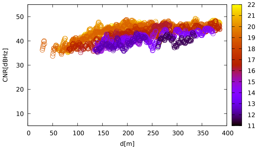
CNR vs distance (LeicaGS15 for E26 at L1)
