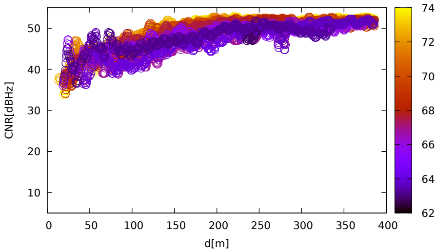
CNR vs distance (LeicaGS15 for E31 at L1)
