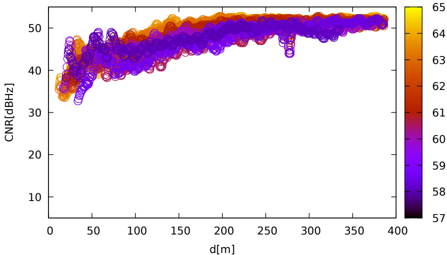
CNR vs distance (LeicaGS15 for E33 at L1)
