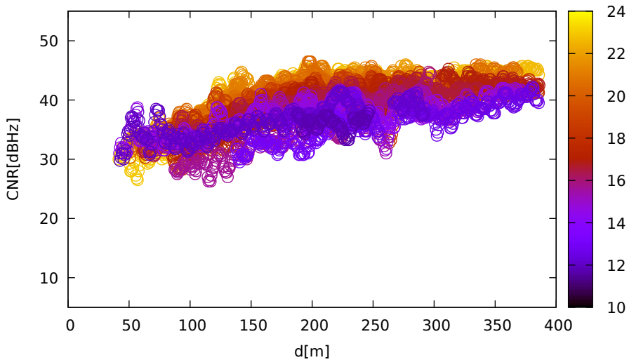
CNR vs distance (LeicaGS15 for G02 at L1)
