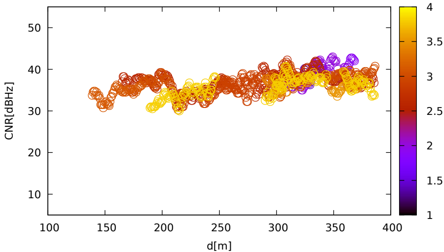
CNR vs distance (LeicaGS15 for G04 at L1)
