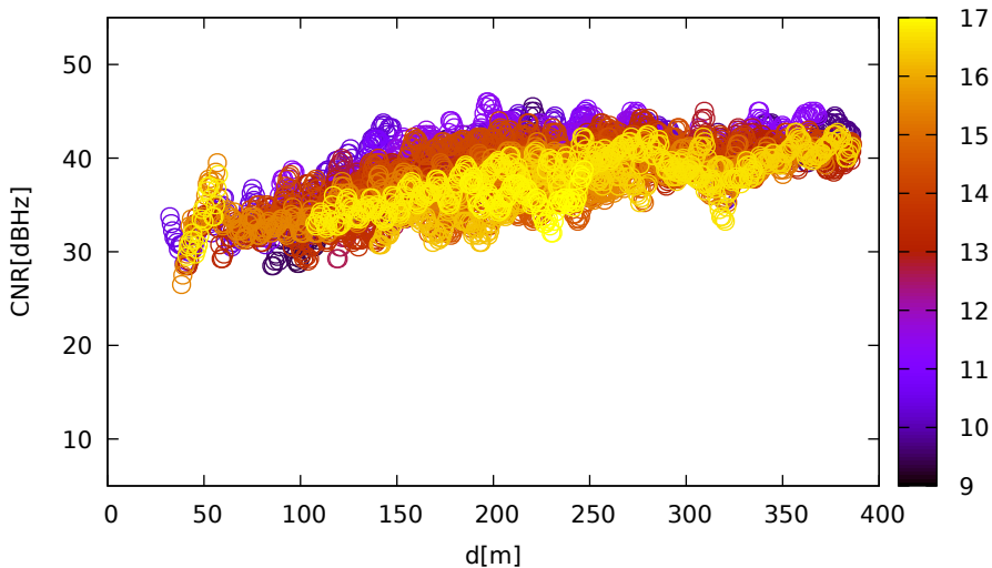
CNR vs distance (LeicaGS15 for G05 at L1)
