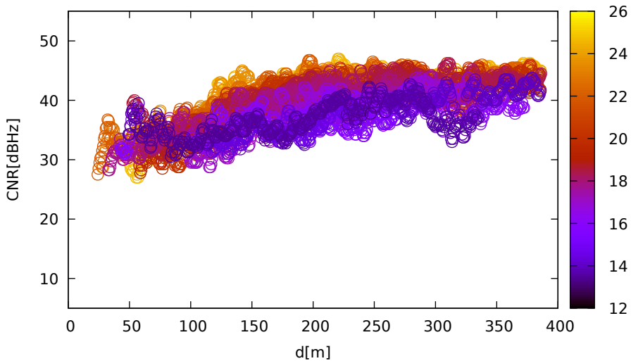
CNR vs distance (LeicaGS15 for G12 at L1)
