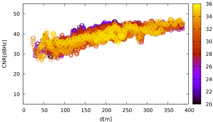
CNR vs distance (LeicaGS15 for G18 at L1)
