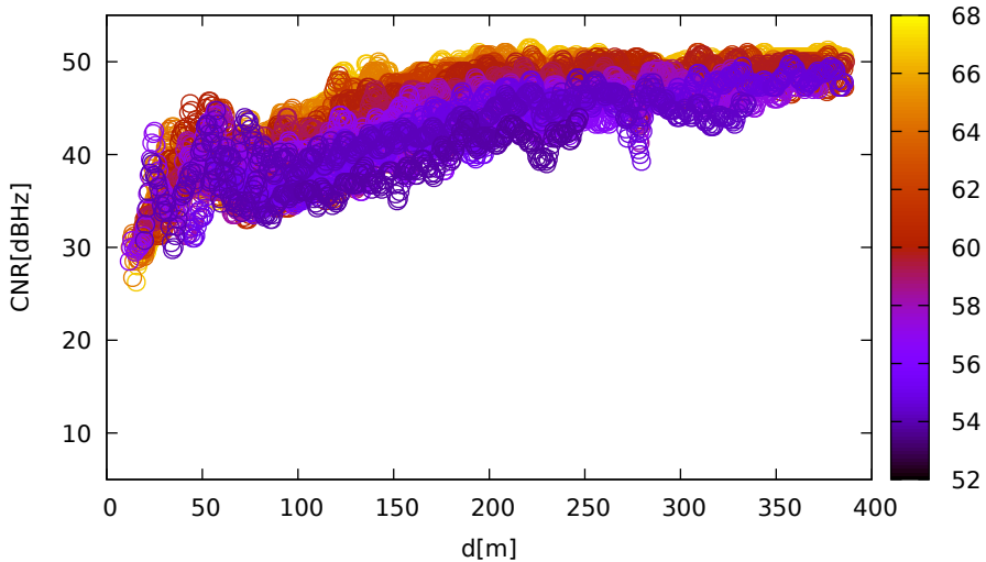
CNR vs distance (LeicaGS15 for G25 at L1)
