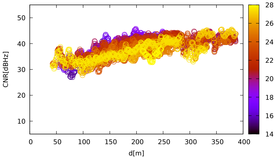
CNR vs distance (LeicaGS15 for G26 at L1)
