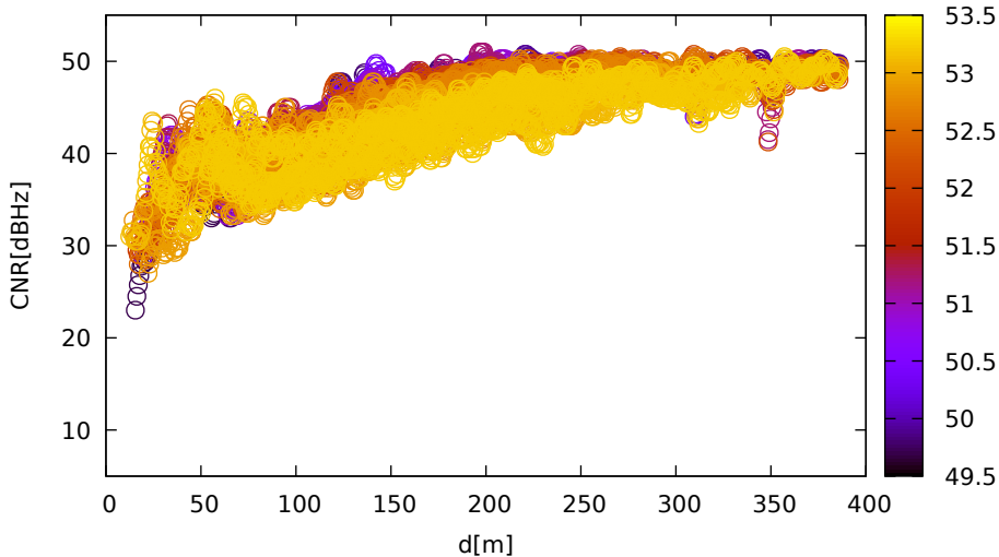
CNR vs distance (LeicaGS15 for G31 at L1)
