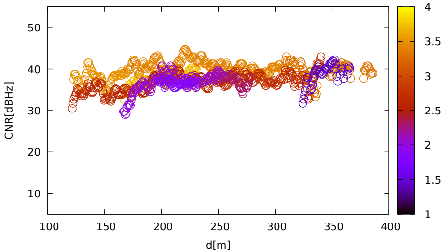
CNR vs distance (LeicaGS15 for G32 at L1)
