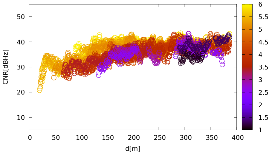
CNR vs distance (LeicaGS15 for R03 at L1)
