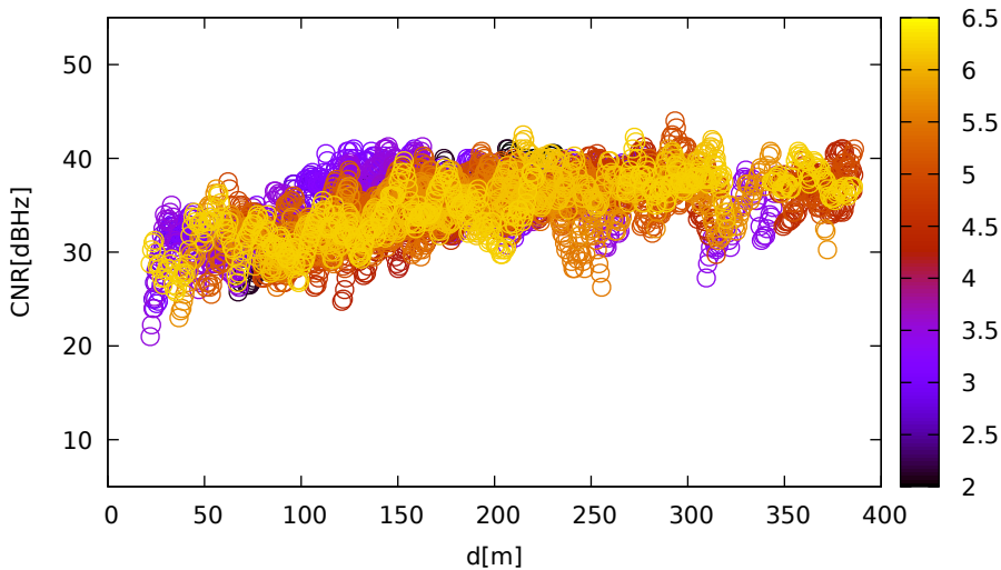
CNR vs distance (LeicaGS15 for R04 at L1)
