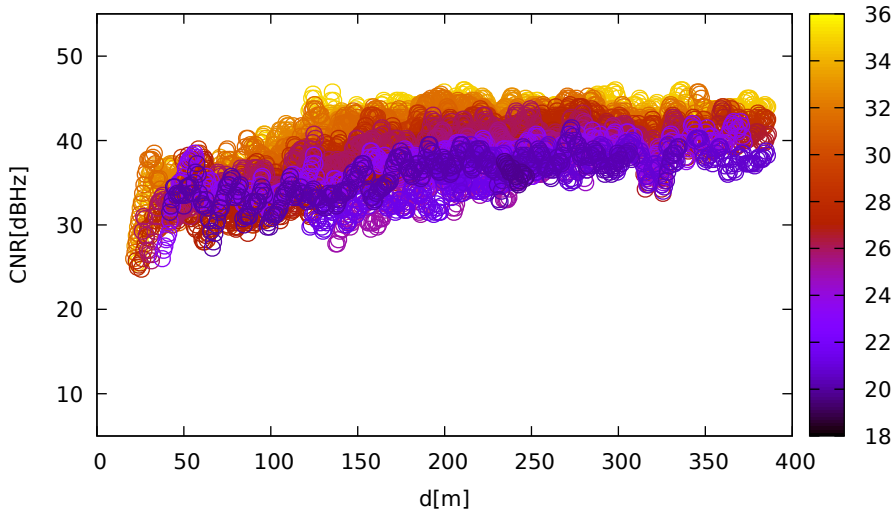
CNR vs distance (LeicaGS15 for R10 at L1)
