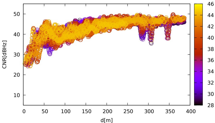
CNR vs distance (LeicaGS15 for R12 at L1)
