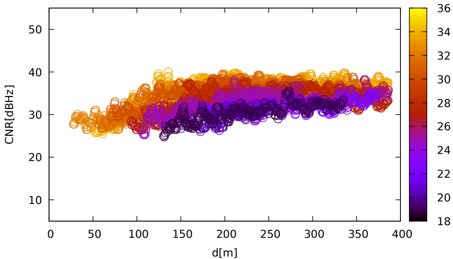
CNR vs distance (LeicaGS15 for R20 at L1)
