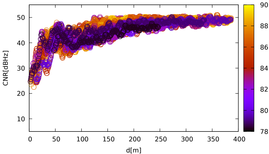
CNR vs distance (LeicaGS15 for R21 at L1)
