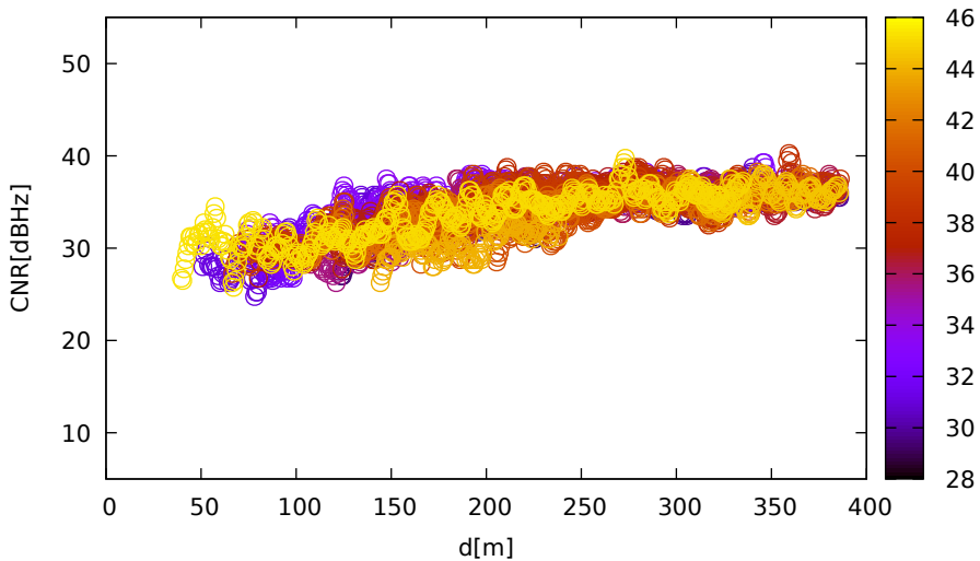
CNR vs distance (LeicaGS15 for R22 at L1)
