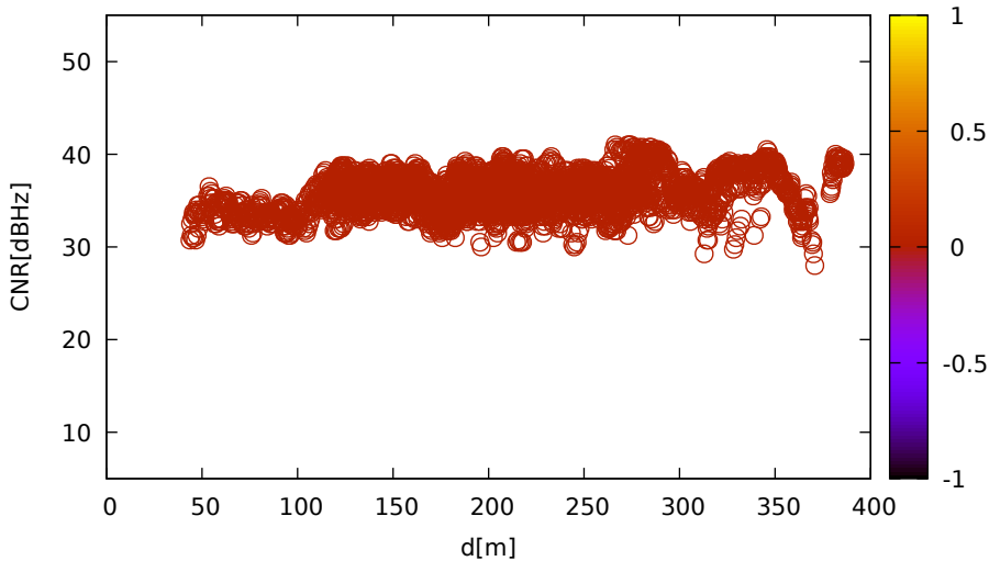
CNR vs distance (LeicaGS18 for C02 at L1)
