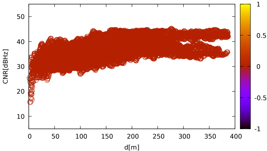
CNR vs distance (LeicaGS18 for C08 at L1)
