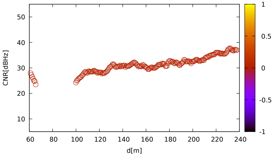
CNR vs distance (LeicaGS18 for C14 at L1)
