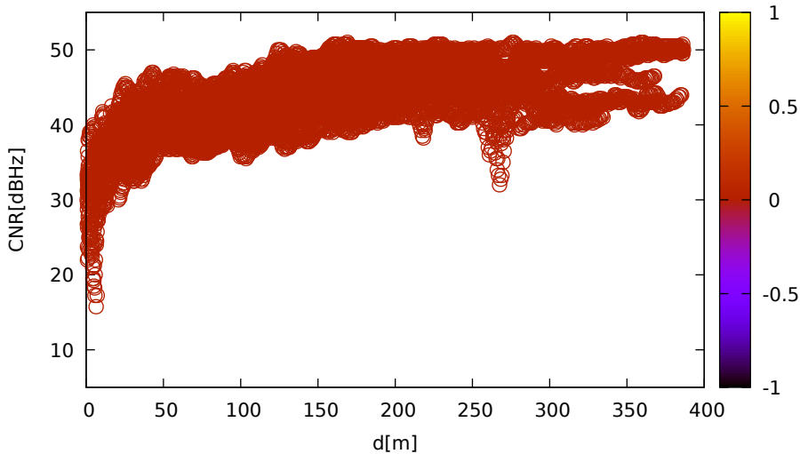
CNR vs distance (LeicaGS18 for C28 at L1)
