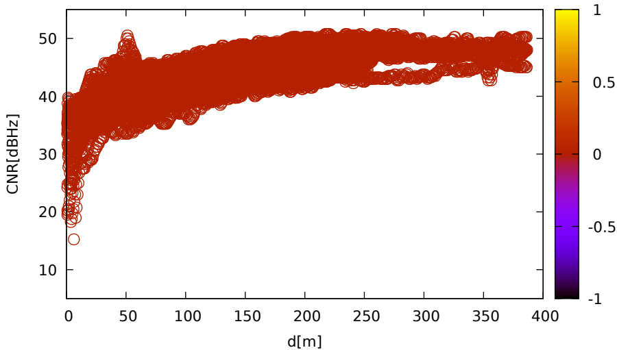
CNR vs distance (LeicaGS18 for C30 at L1)
