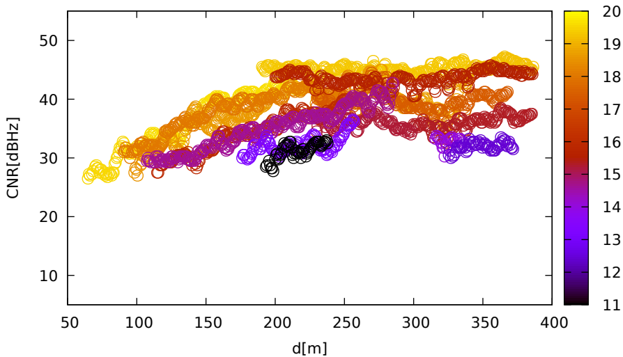
CNR vs distance (LeicaGS18 for E01 at L1)
