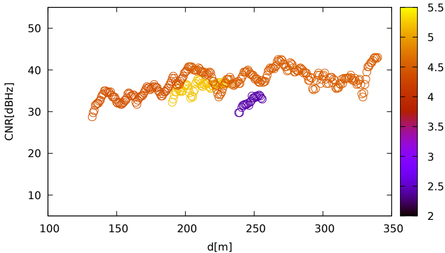
CNR vs distance (LeicaGS18 for E05 at L1)
