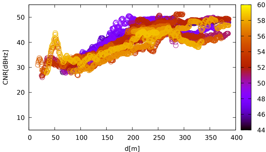
CNR vs distance (LeicaGS18 for E12 at L1)
