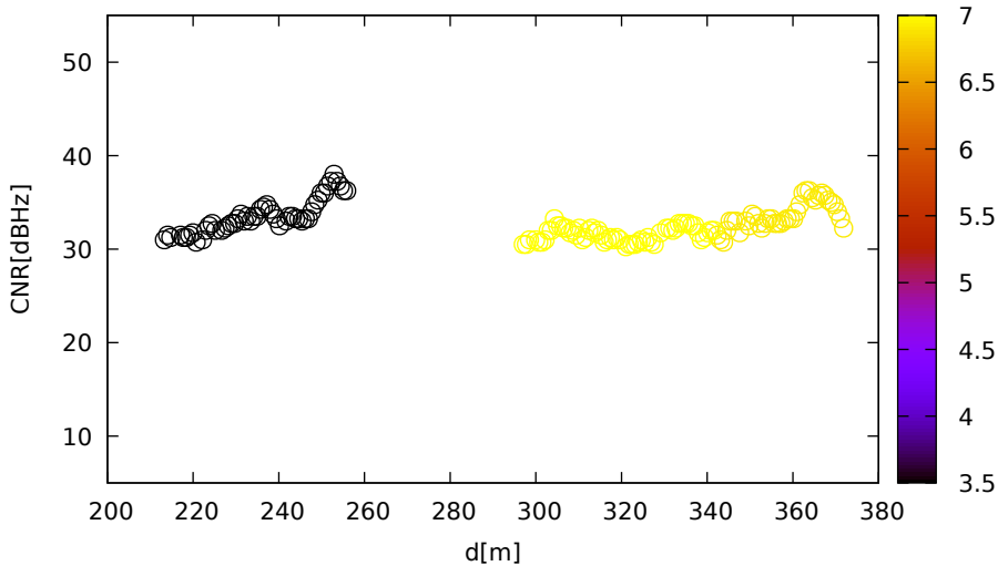
CNR vs distance (LeicaGS18 for E25 at L1)
