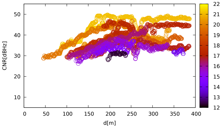
CNR vs distance (LeicaGS18 for E26 at L1)
