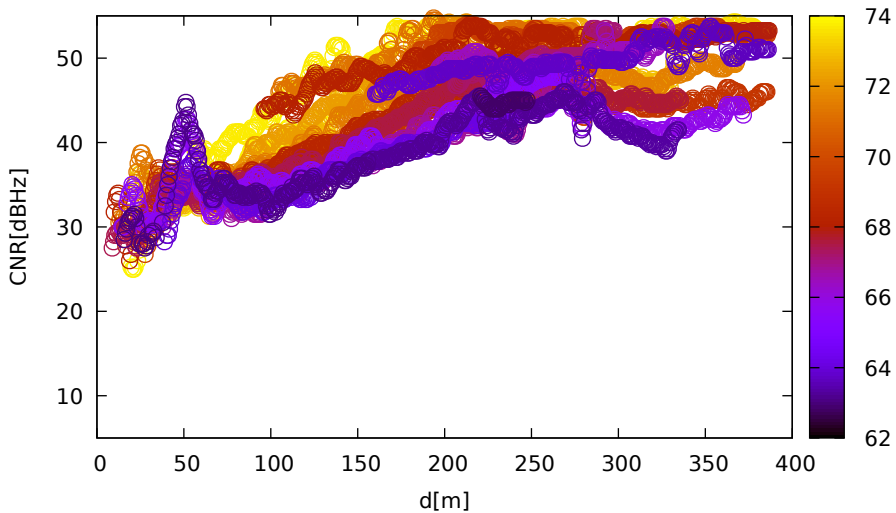
CNR vs distance (LeicaGS18 for E31 at L1)
