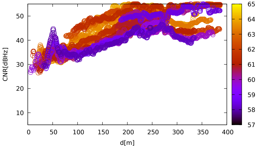
CNR vs distance (LeicaGS18 for E33 at L1)
