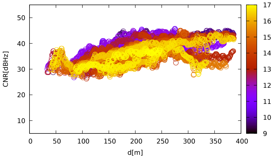
CNR vs distance (LeicaGS18 for G05 at L1)
