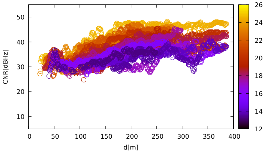
CNR vs distance (LeicaGS18 for G12 at L1)
